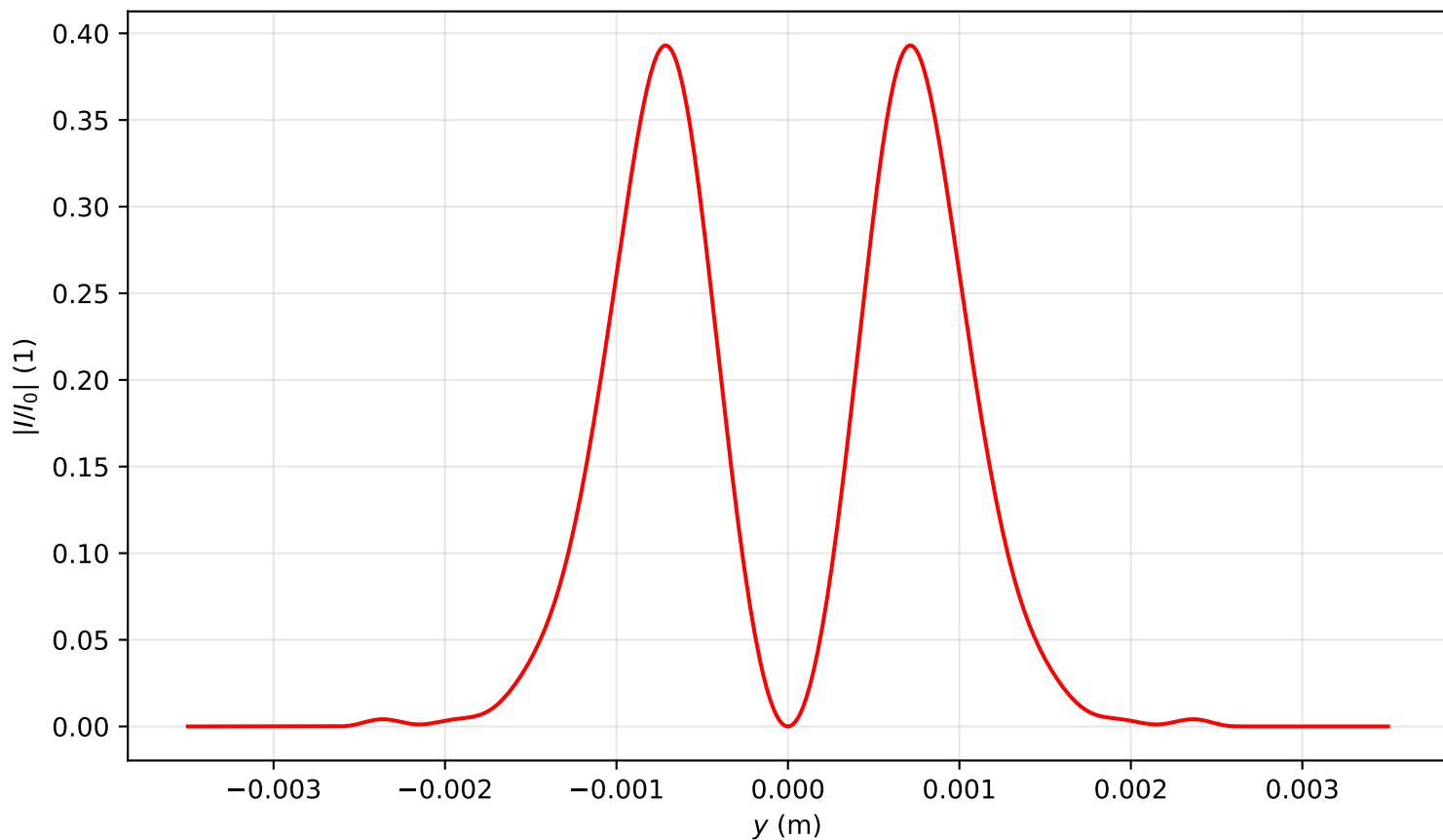
Intensity profile I(x=0, y, z=2.627)/I_0 , P_{in}=3.0P_{cr} , artificial time
